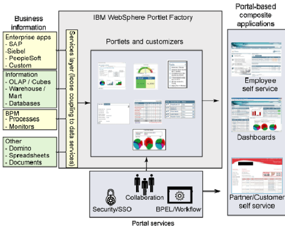
Figure 1. Web Experience Factory application architecture
